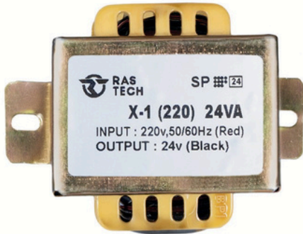
TRANSFORMER X-1 SP (220) MRP - 630/-
